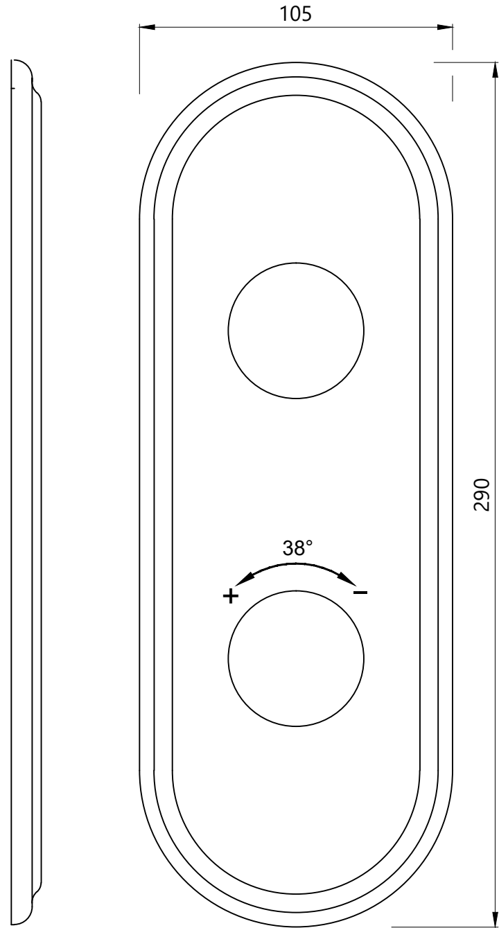
WALL FLANGE
